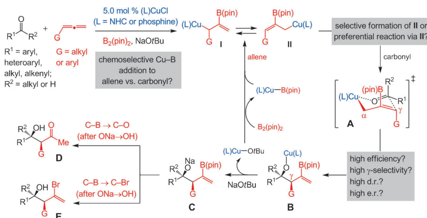
Scheme 1. Chemoselective Cu–B addition to an allene, followed by site-, diastereo-, and enantioselective addition of the resulting 2-(pinacolato)boron-substituted allylcopper species to aldehydes and ketones can lead to a range of valuable organic molecules by a catalytic multicomponent operation. B(pin) = (pinacolato)boron, L = ligand.
